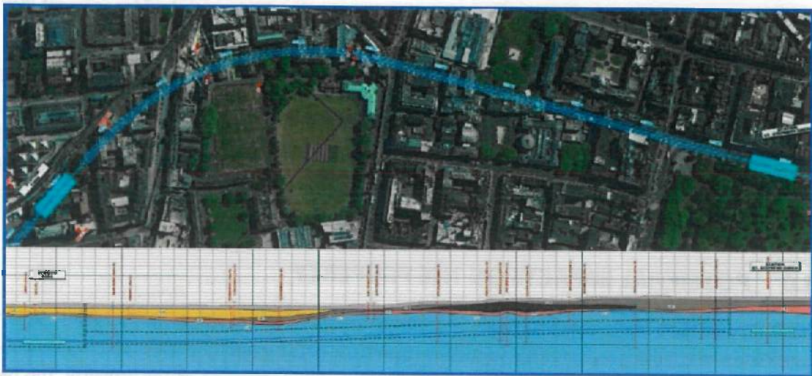
Figure 12. Geological Section (ref. A5.13, Diagram 3.13: Geologic Profile for TBM Drive C8- Tara Station to St. Stephen's Green)
