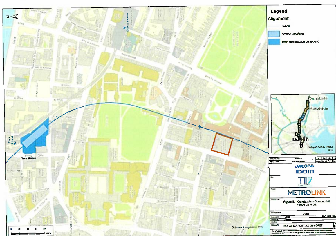
Figure 11. Plan showing horizontal alignment (extract from ML1-JAI-EIA-ROUT_XX-DR-Y-05025)
