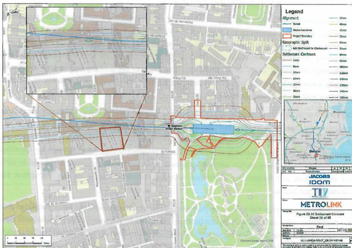
Figure 13. Settlement Contours (Extract from ML1-JAI-EIA-ROUT_XX-DR-Y-21148)
